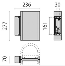
000422 Wall bracket 27
